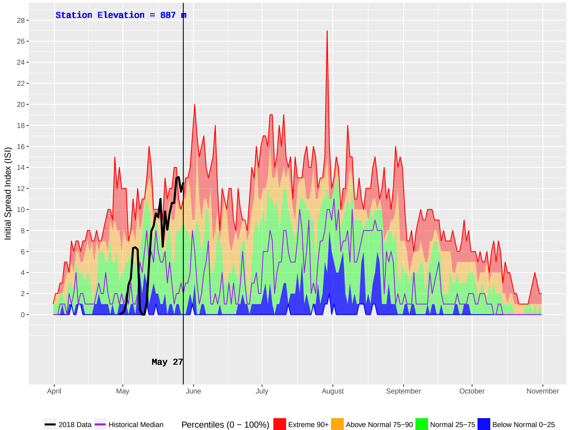
CRAWFORD (873) : Historical (2004–2016) and Current (2018) Noon Initial Spread Index (ISI)
