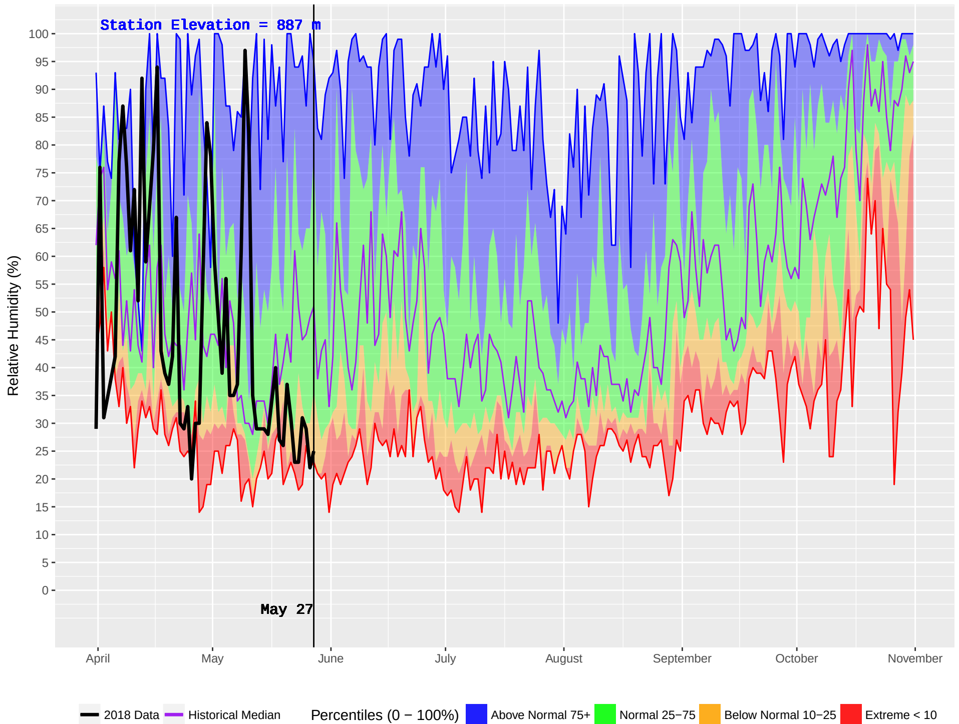
CRAWFORD (873) : Historical (2004–2016) and Current (2018) Noon Relative Humidity
